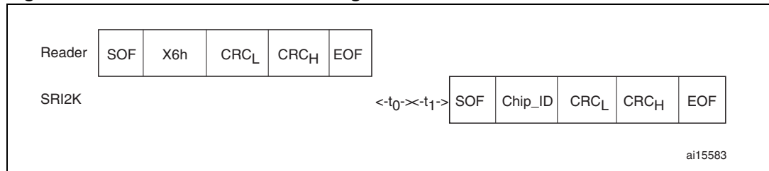
Figure 54. Slot_marker frame exchange between reader and SRI2K
