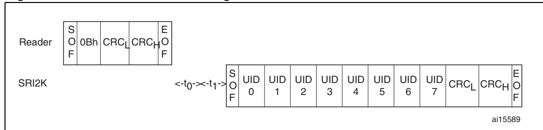
Figure 60. Get_UID frame exchange between reader and SRI2K
