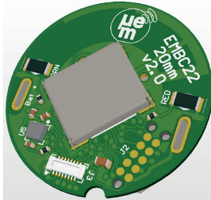
Figure 1: Accelerometer beacon module PCB with connector
