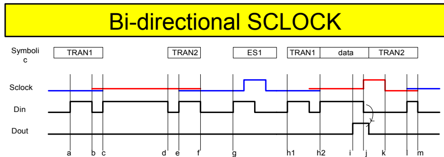
Figure 18 Bi-directional SCLOCK
