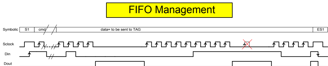
Figure 16 FIFO Management
