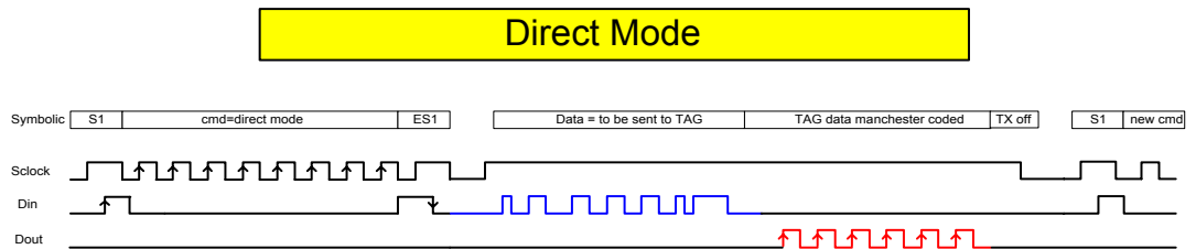
Figure 13 Direct Mode
