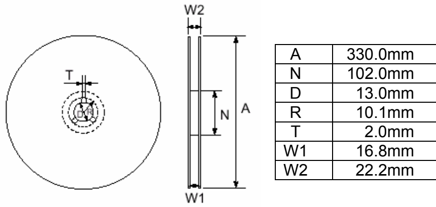
Figure 3 Reel Dimensions
