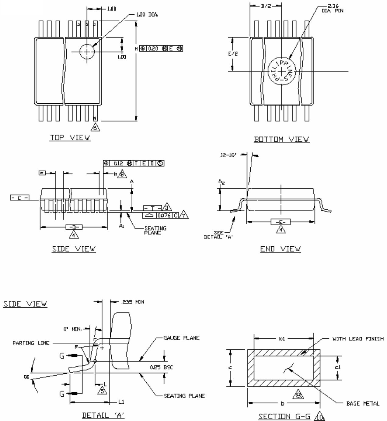
Figure 7 Mechanical Construction
