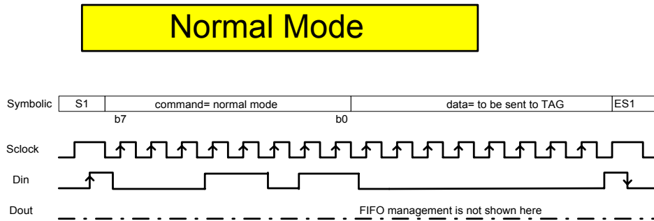
Figure 11 Normal Mode
