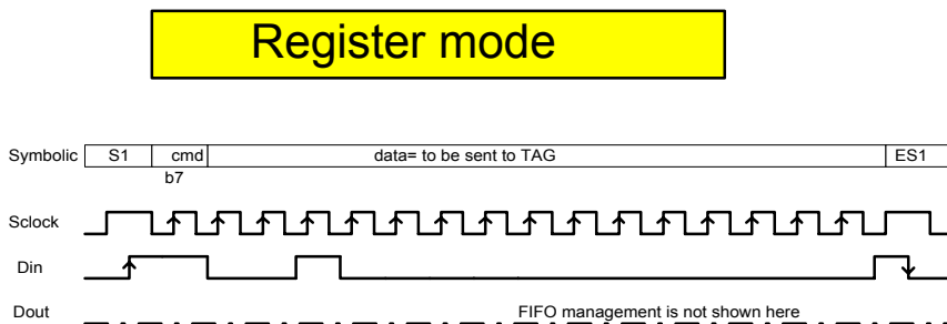
Figure 12 Register Mode
