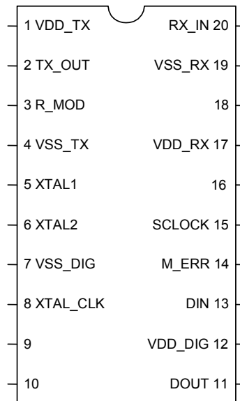
Figure 5 Transceiver Pins
