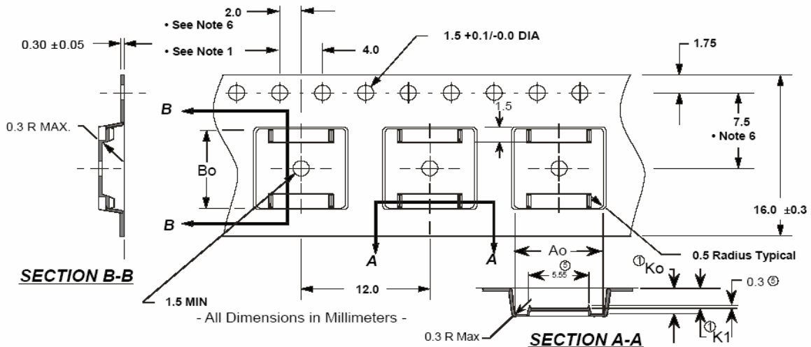
Figure 2 Tape Dimensions
