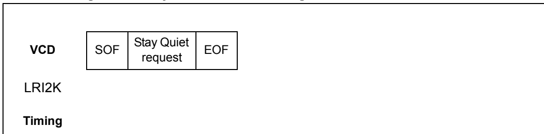
Figure 40. Stay Quiet frame exchange between VCD and LRI2K
