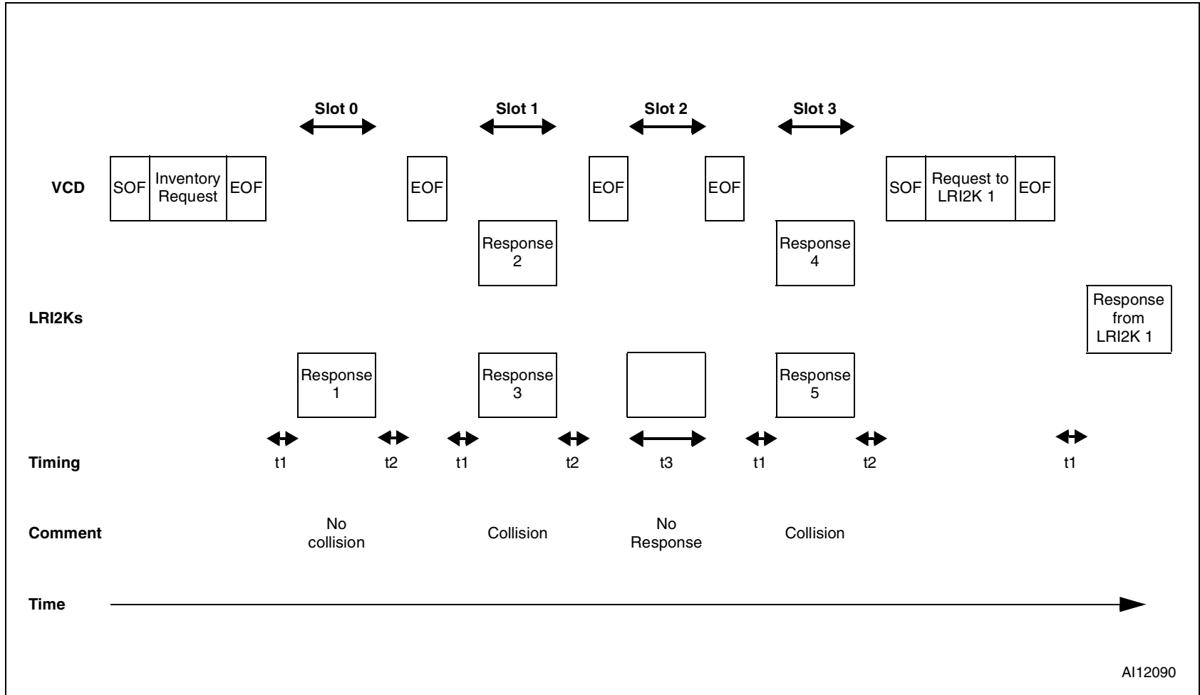
Figure 39. Description of a possible anticollision sequence
