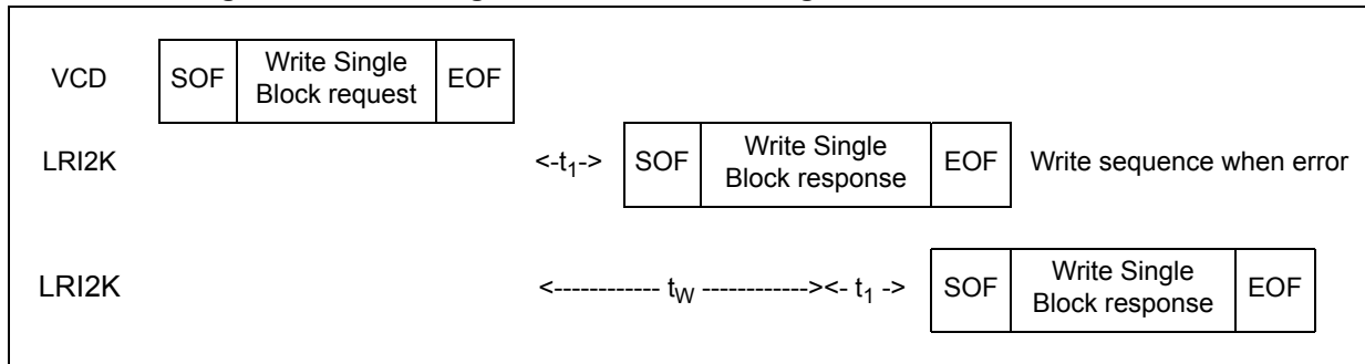
Figure 42. Write Single Block frame exchange between VCD and LRI2K
