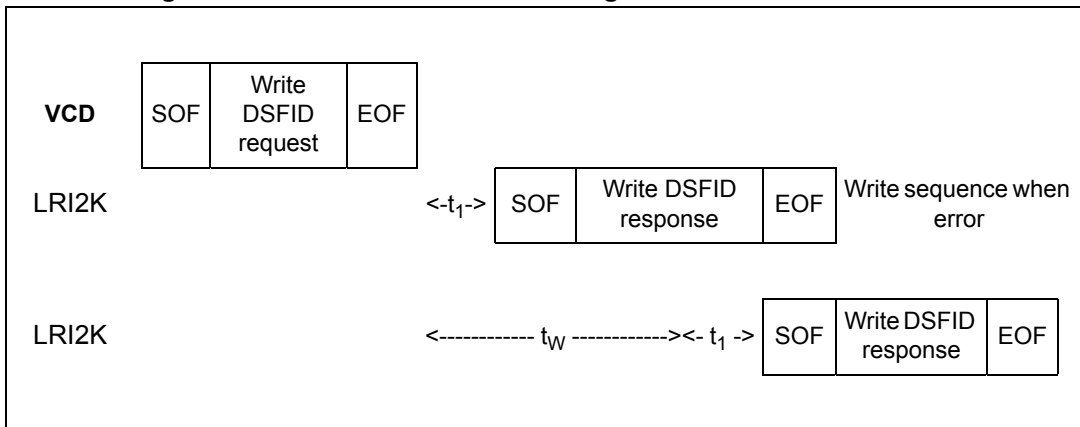
Figure 49. Write DSFID frame exchange between VCD and LRI2K
