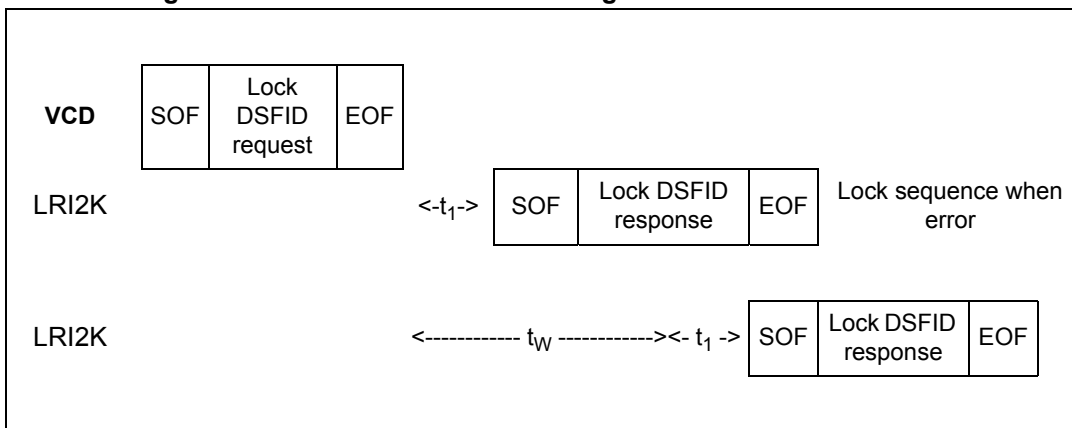
Figure 50. Lock DSFID frame exchange between VCD and LRI2K
