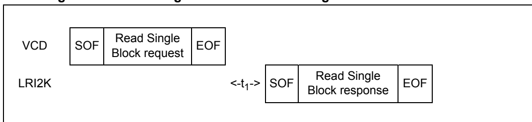
Figure 41. READ Single Block frame exchange between VCD and LRI2K
